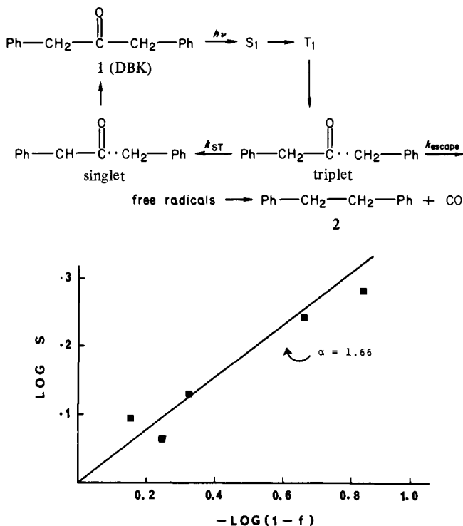
Figure 1. 13 C content of recovered dibenzyl ketone (DBK). Plot of separation factor, S , vs. fraction, f , of reacted DBK.
